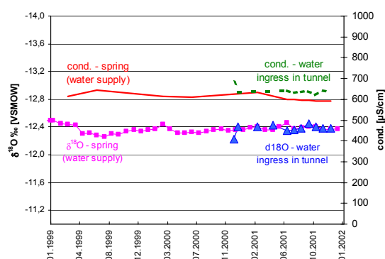
Figure 1. \delta^{18}\text{O} -Values and electrical conductivity from the spring and the water ingress in tunnel
