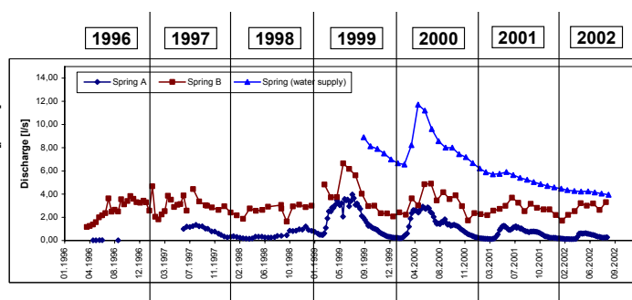
Figure 2. Long-term spring discharge hydrographs from the Lower Inn Valley, Austria
