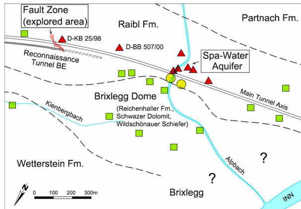
Figure 3. Schematic Map showing known area of fault zone and measuring points locations classified with respect to the response of the draw-down (triangles = reaction water level/discharge and electric conductivity; circles = reaction electric conductivity, squares = no reaction)
